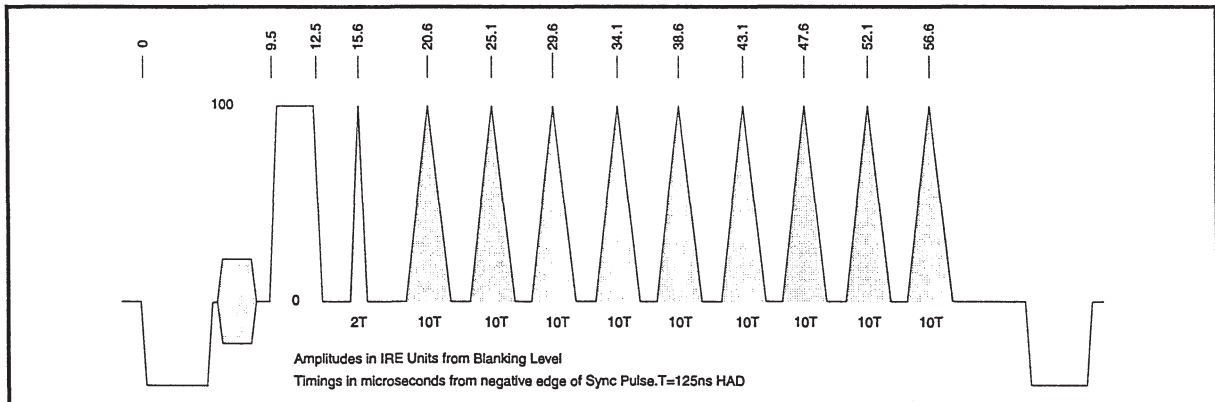
Colour Multipulse 525
