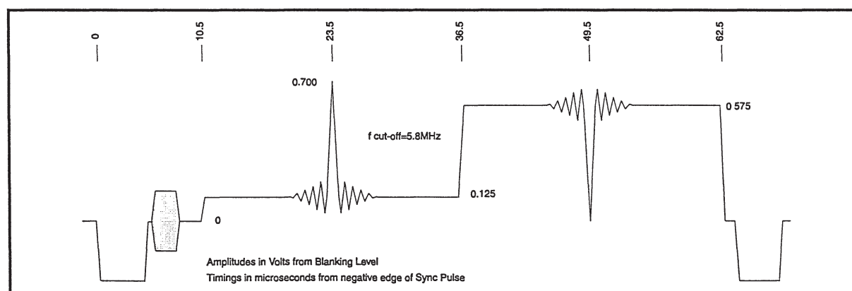
Sinx/x 625 PAL
